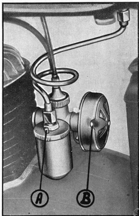
Obr. 4 Splynovač
